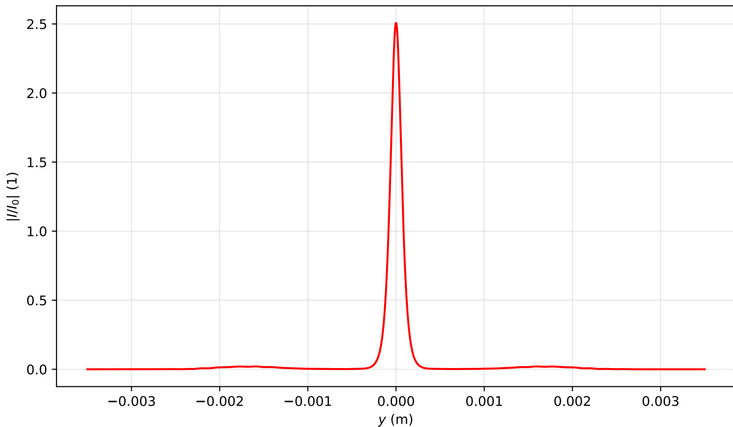
Intensity profile I(x=0, y, z=1.274)/I_0 , P_{in}=6.0P_{cr} , artificial time
